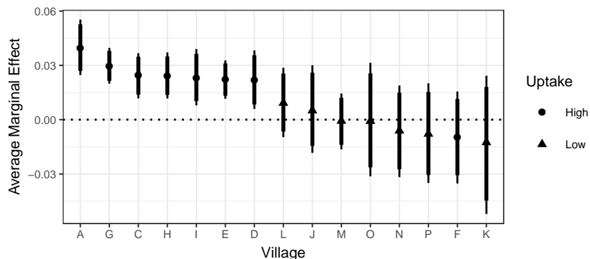
Figure 5: Average marginal effect of one adopting neighbor on adoption by village. Estimates from a multilevel model suggest that save for village F, high uptake villages have large, significant peer effects. Low uptake villages have small, statistically insignificant peer effects. Village B is omitted because its sample size is too small.
