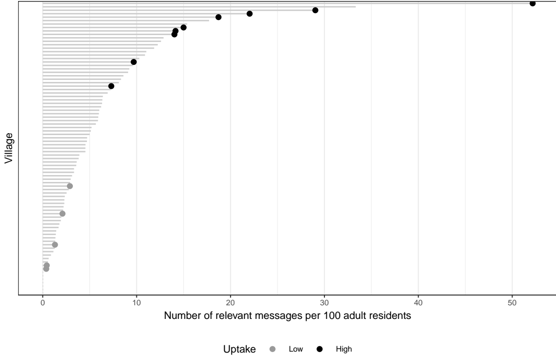
Figure 1: Number of relevant messages (normalized) by village.
