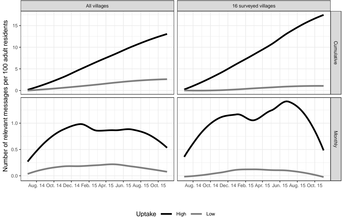
Figure 2: Message intensity over time. The monthly (bottom-panel) and cumulative (top) number of relevant messages overtime per 100 residents, smoothed using a Loess fit. Villages in the left panel are clustered using a Gaussian mixture model with two mixture components (see SI, Section 2.2 for additional details).
