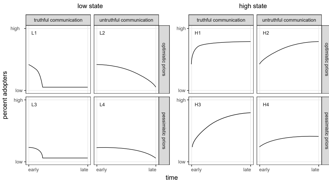
Figure 3: Illustration of main model propositions. Initial adoption depends on priors (Theorem 1). Truthful communication enables peer effects (proposition 5) that allow matching the state faster (proposition 2).
