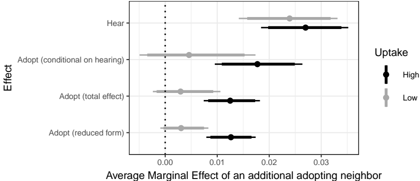
Figure 6: Selection model with hearing. Average marginal effect of an adopting neighbor on hearing (first stage) and of adopting conditional on hearing (second stage). Peers impact hearing about the innovation in both high- and low-uptake villages. Yet, only in high-uptake villages do peers also affect the likelihood of adopting it conditional on hearing about it. The selection model’s total effect matches the estimate from a reduced form logistic regression (see SI, section 6.1 for details about estimation).
